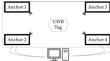
Fig. 3. Overview of UWB system
